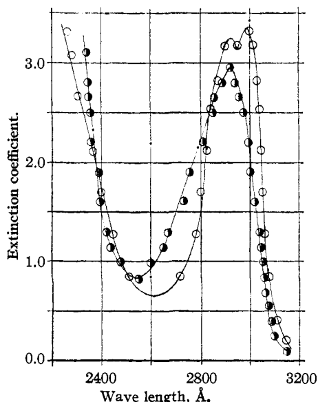
Fig. 1.—Ultraviolet absorption of \alpha -tocopherol in ethanol, one millimole per liter: ●, this \alpha -tocopherol; ○, authentic \alpha -tocopherol.
